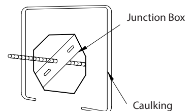
Fig. 3 Sealing
