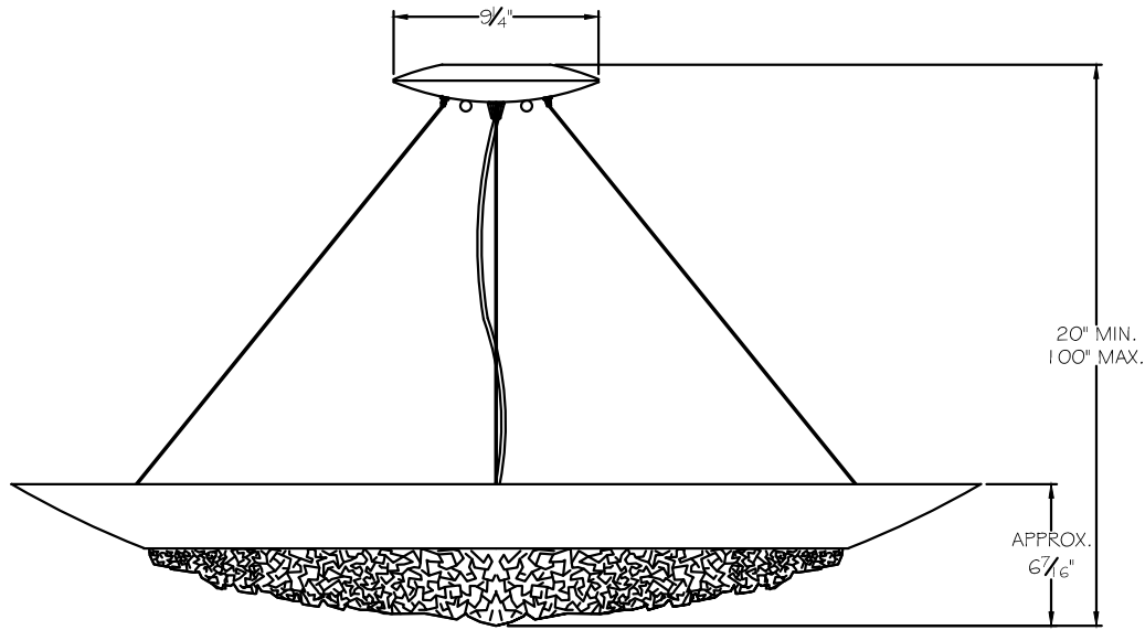
FRONT VIEW
