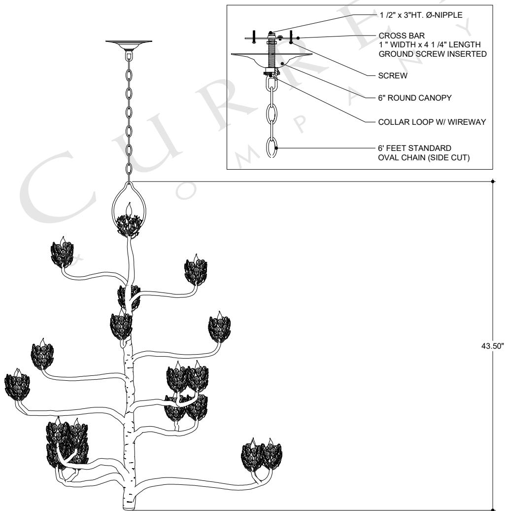
FRONT VIEW
