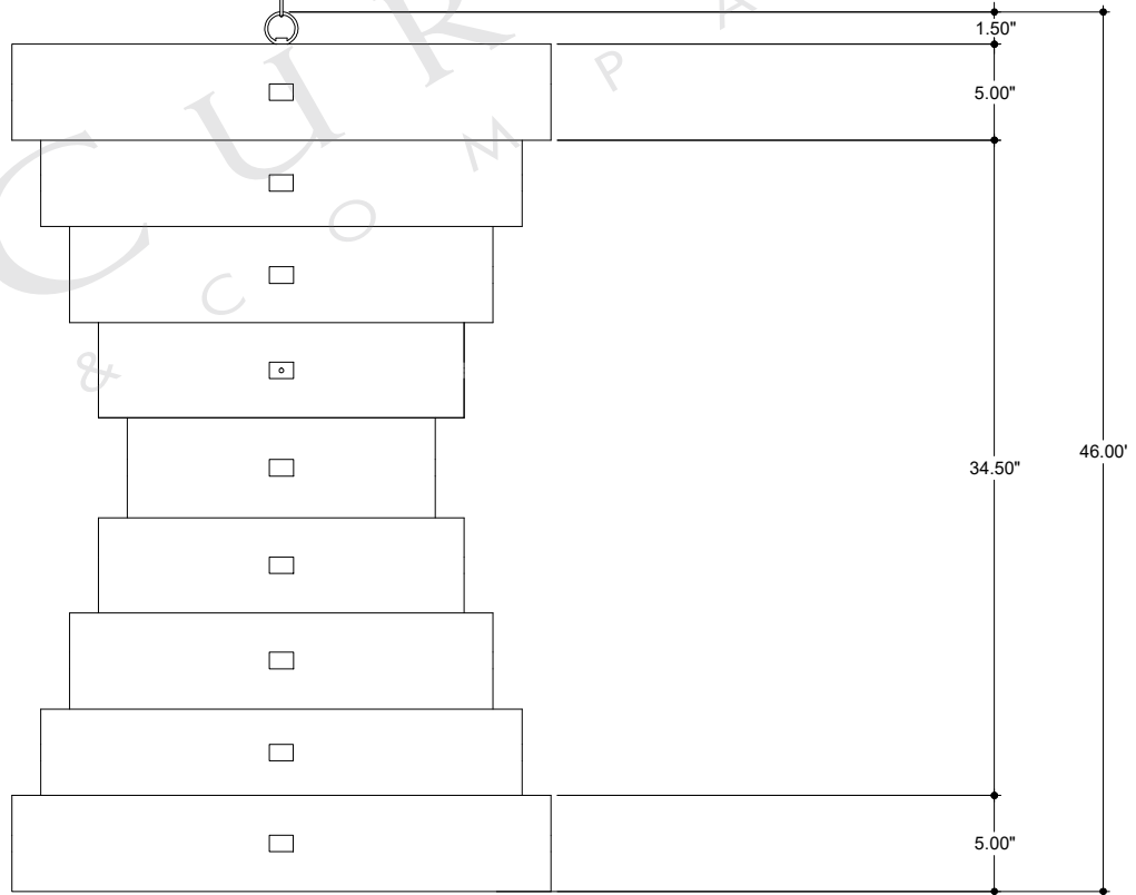
FRONT VIEW
