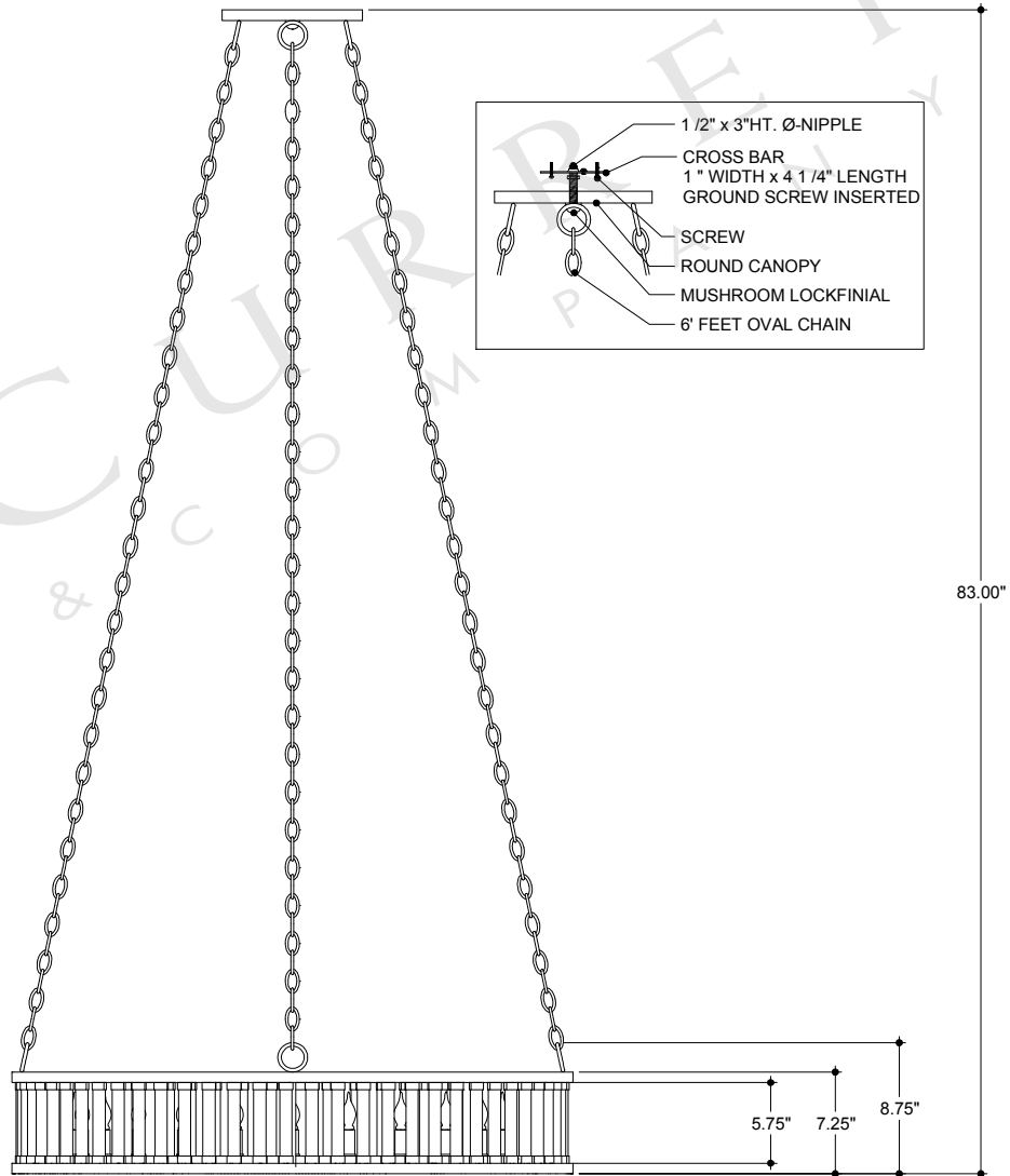
FRONT VIEW
