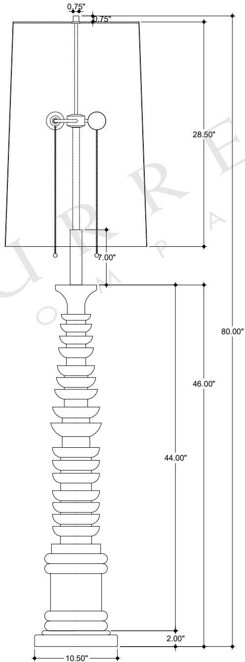
FRONT VIEW
