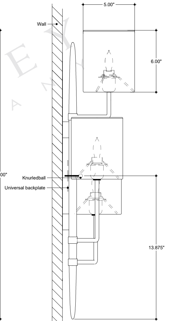
SIDE VIEW
